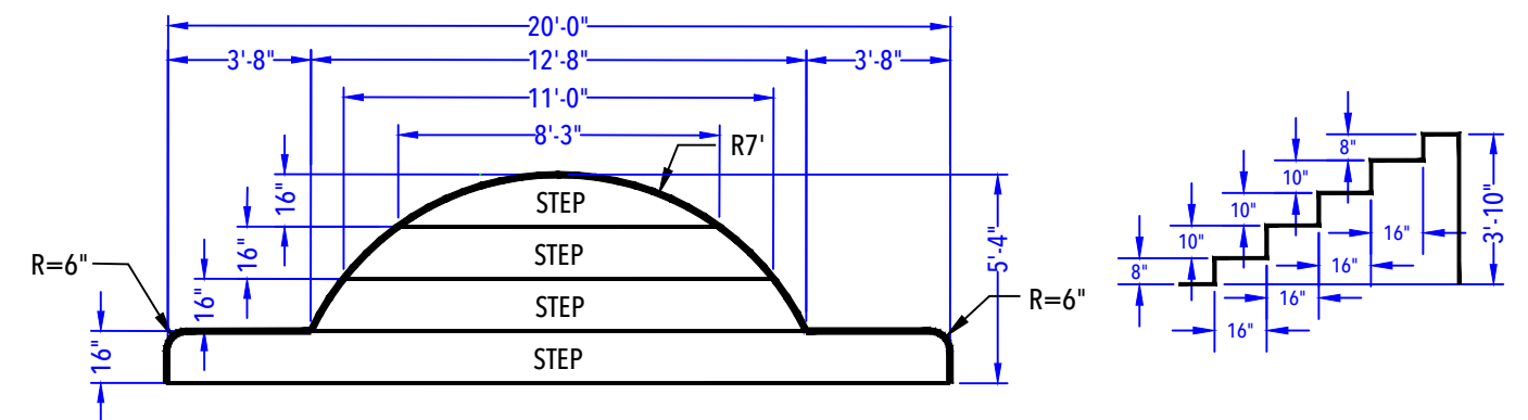
ENTRY STEP DETAIL (After Concrete & Liner) N.T.S.
