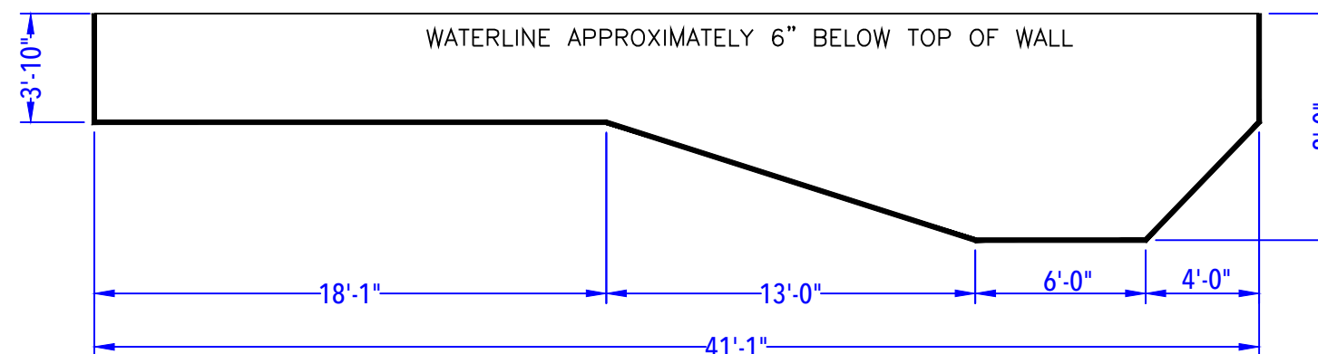
DEPTH DETAIL
