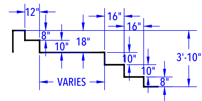
SUN DECK & ENTRY STEP DETAIL (After Concrete & Liner) N.T.S.
