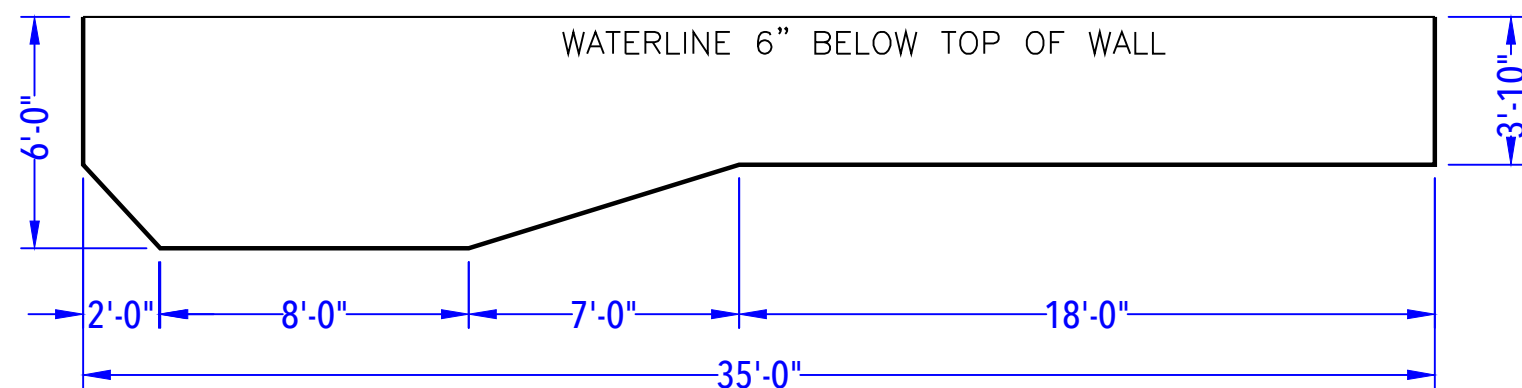
DEPTH DETAIL
