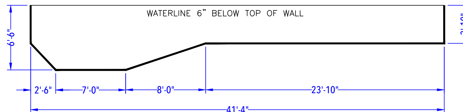
DEPTH DETAIL
