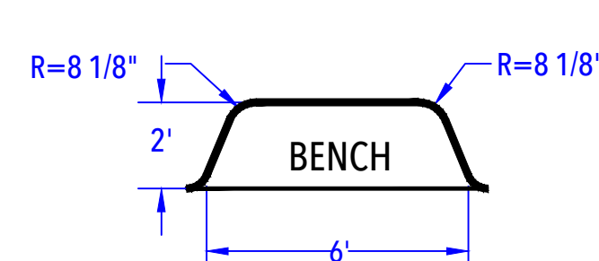
DEEP END BENCH DETAIL (After Concrete & Liner) N.T.S.
