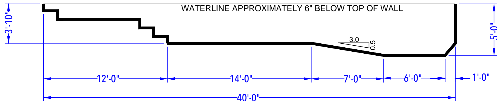
DEPTH DETAIL
