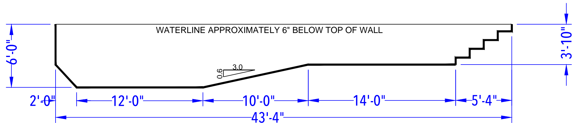
DEPTH DETAIL
