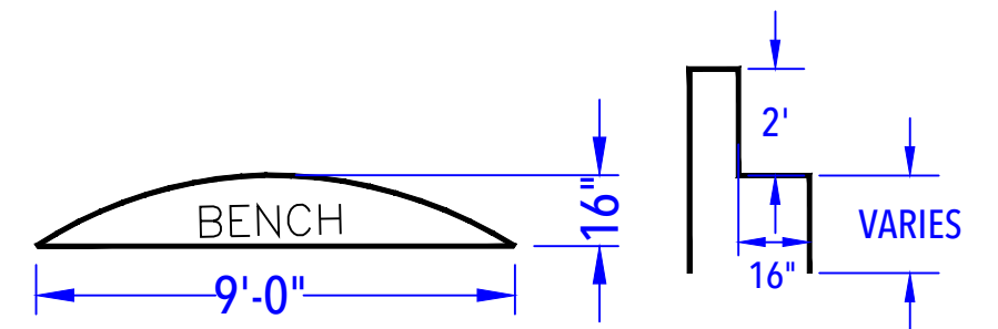
DEEP END BENCH DETAIL (After Concrete & Liner) N.T.S.
