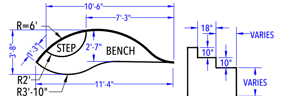
DEEP END BENCH & STEP OUT DETAIL (After Concrete & Liner)
