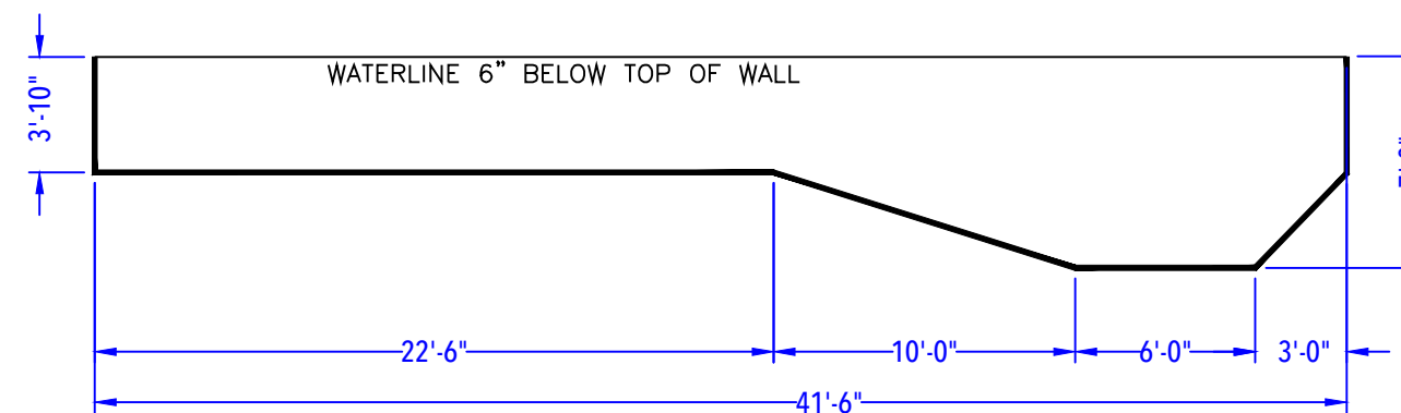
DEPTH DETAIL
