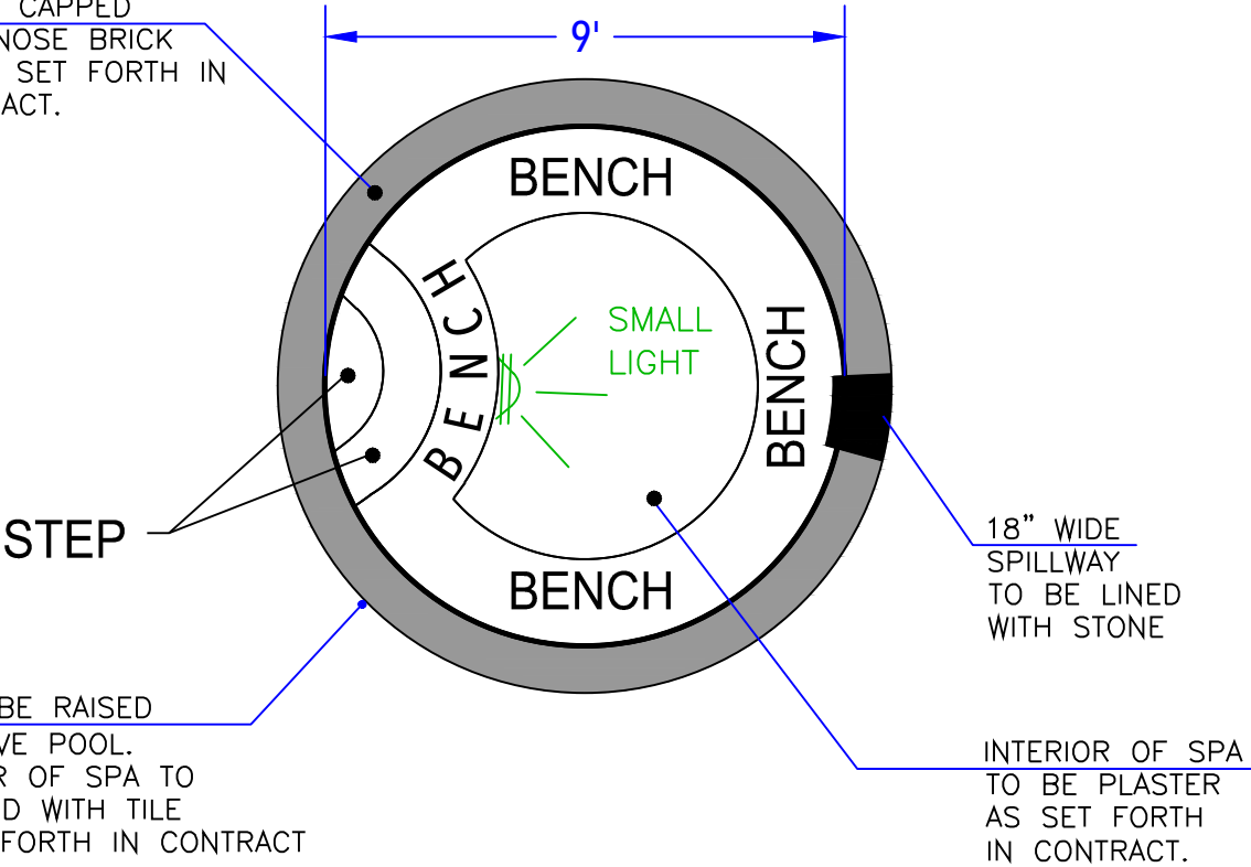
SPA PLAN VIEW (After Concrete & Plaster) N.T.S.
