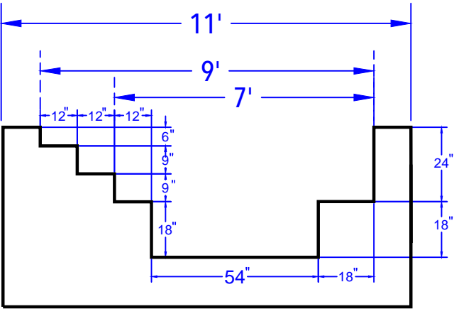
SPA ELEVATION VIEW (After Concrete & Plaster) N.T.S.
