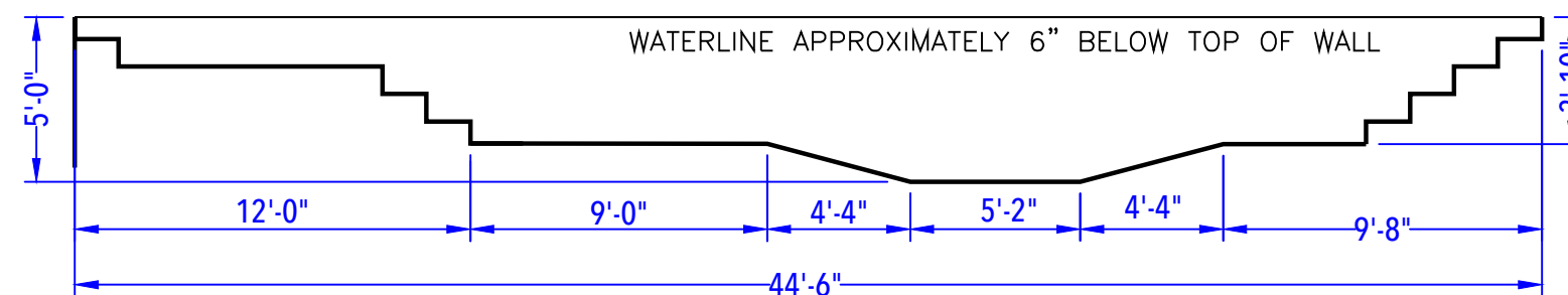
DEPTH DETAIL
