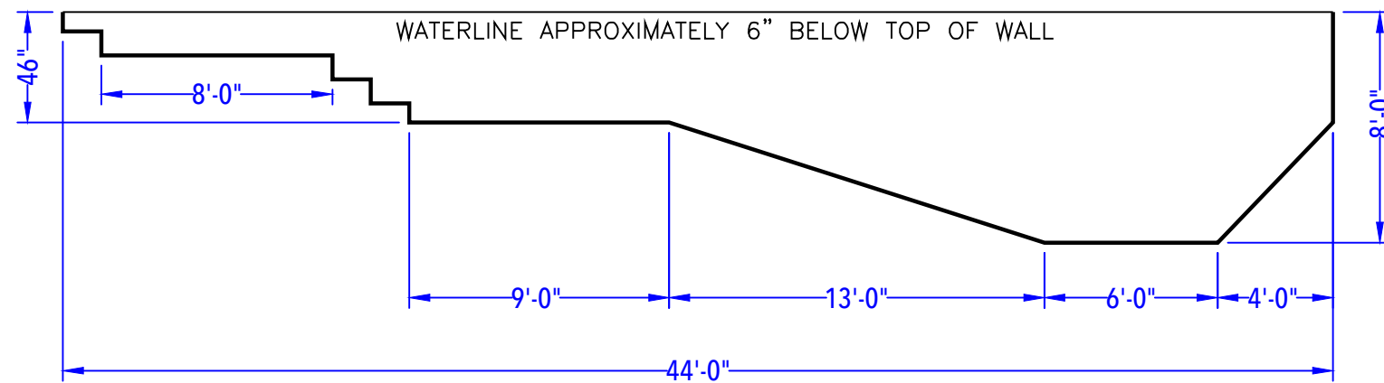
DEPTH DETAIL
