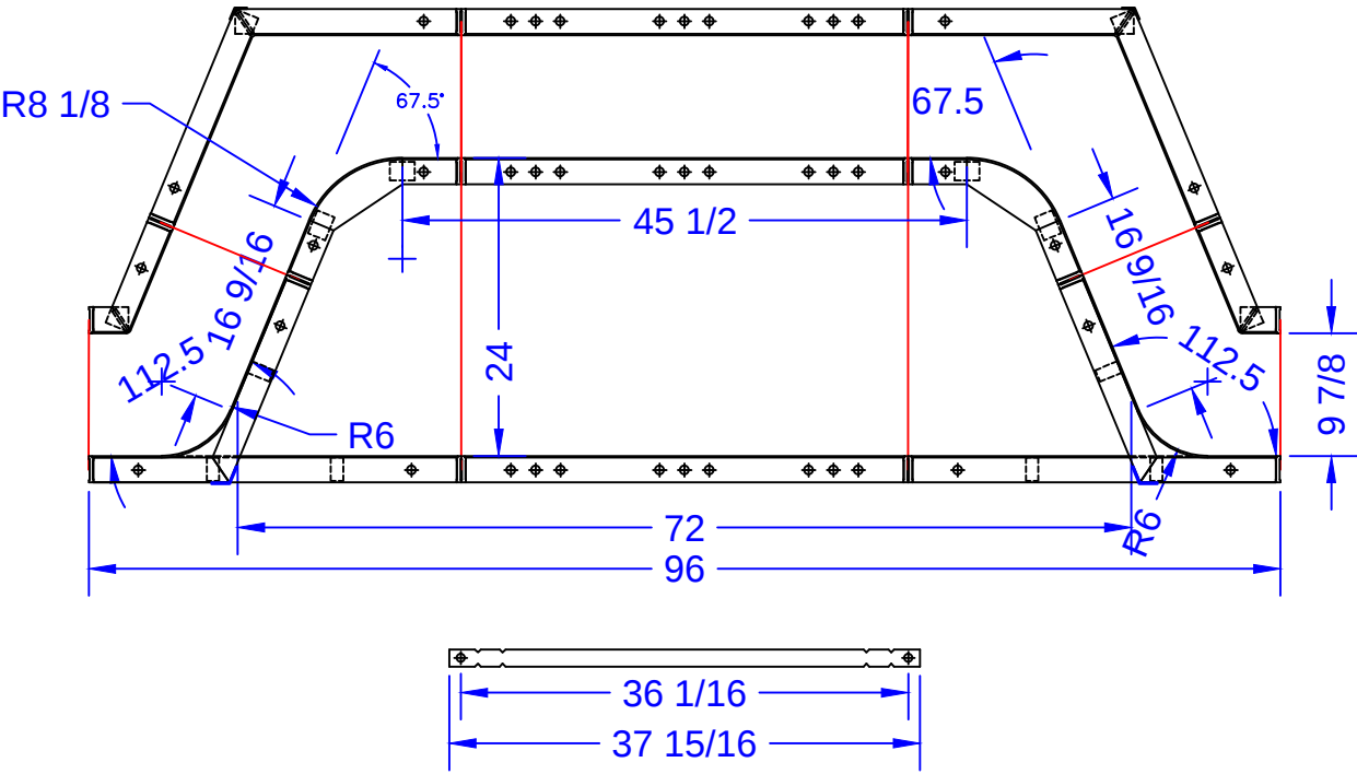
6' Bench Assembly
