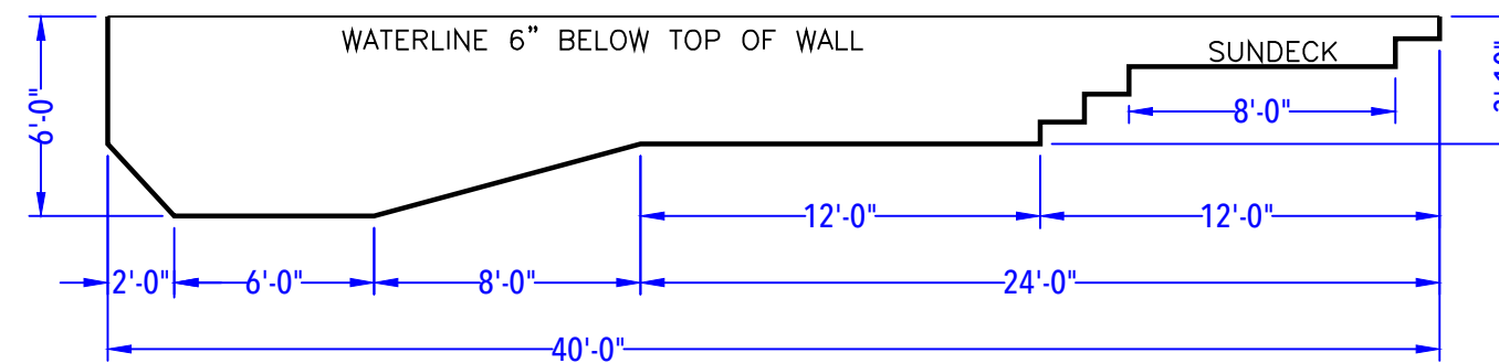
DEPTH DETAIL
