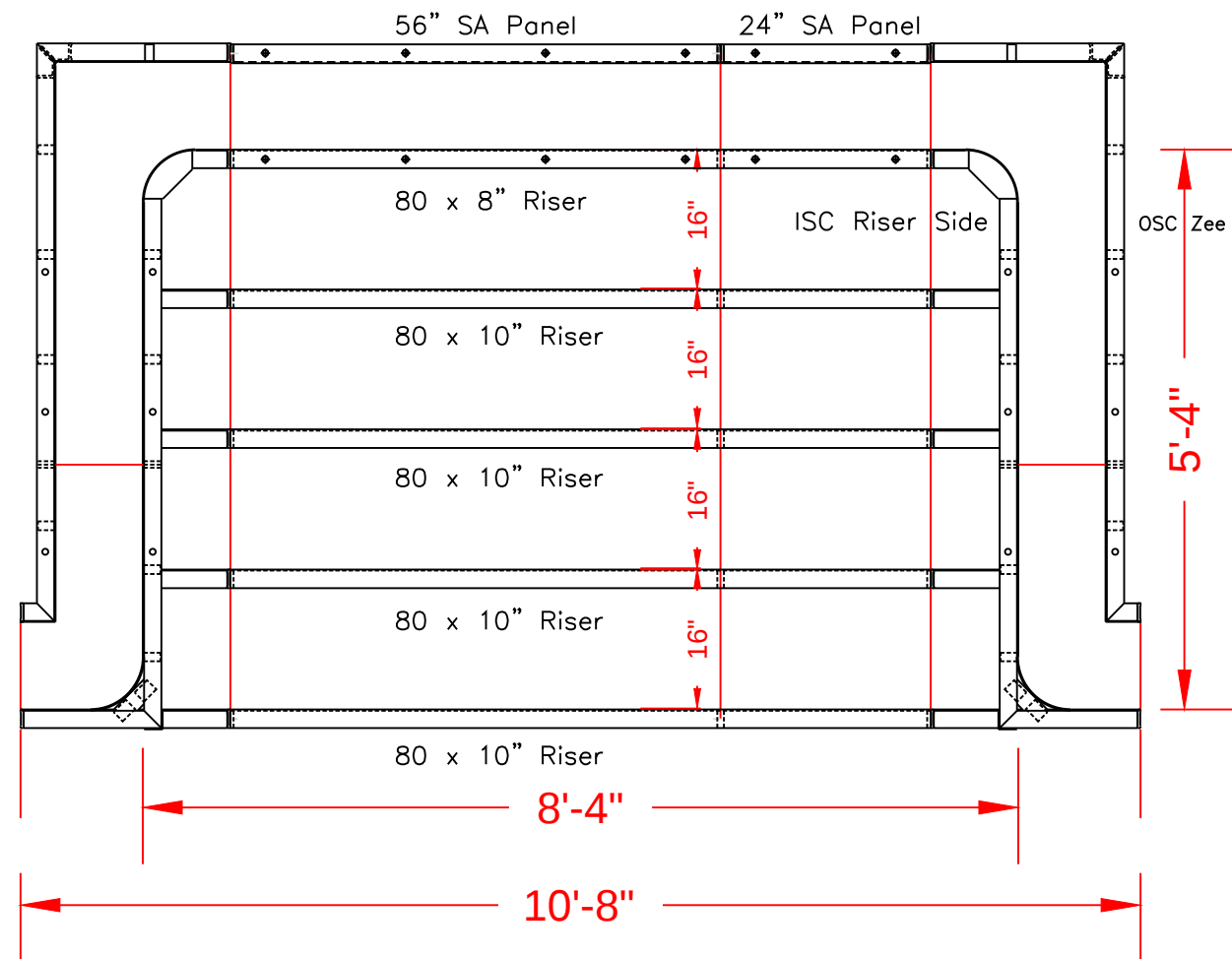
8'-4" x 5'-4" WIDE STEP DETAIL
