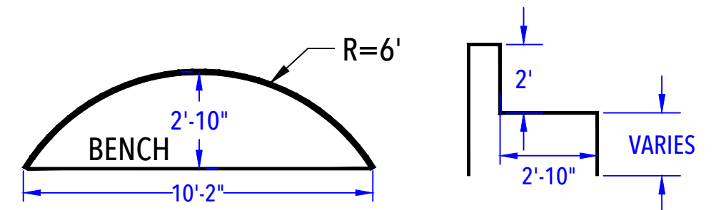
DEEP END BENCH DETAIL (After Concrete & Liner) N.T.S.
