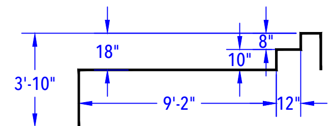
SIDE SUN DECK DETAIL (After Concrete & Liner) N.T.S.
