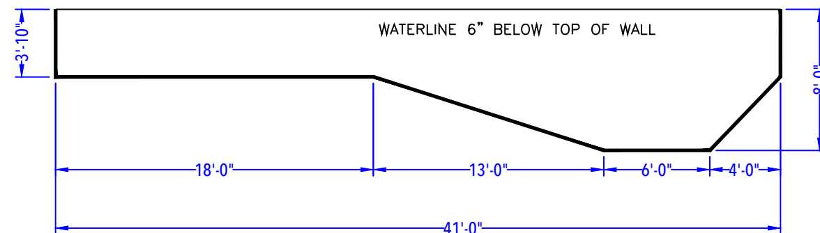
DEPTH DETAIL
