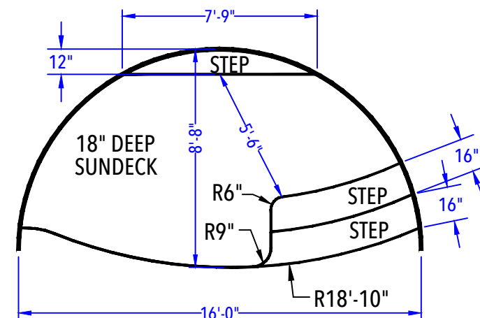
SUN DECK & ENTRY STEP DETAIL (After Concrete & Liner) N.T.S.
