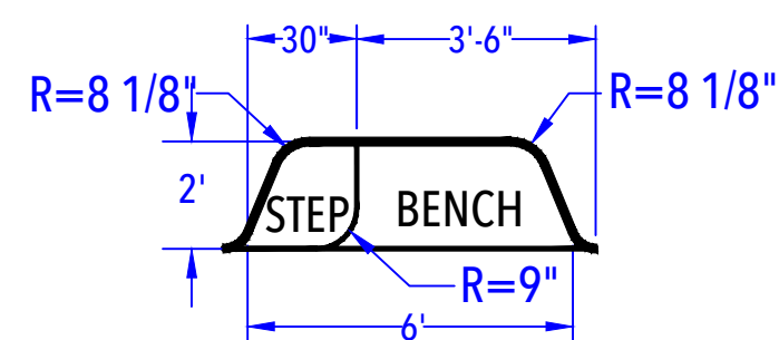
DEEP END BENCH & STEP OUT DETAIL (After Concrete & Liner) N.T.S.
