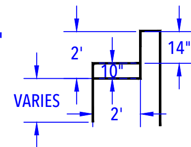
DEEP END BENCH & STEP OUT DETAIL (After Concrete & Liner) N.T.S.
