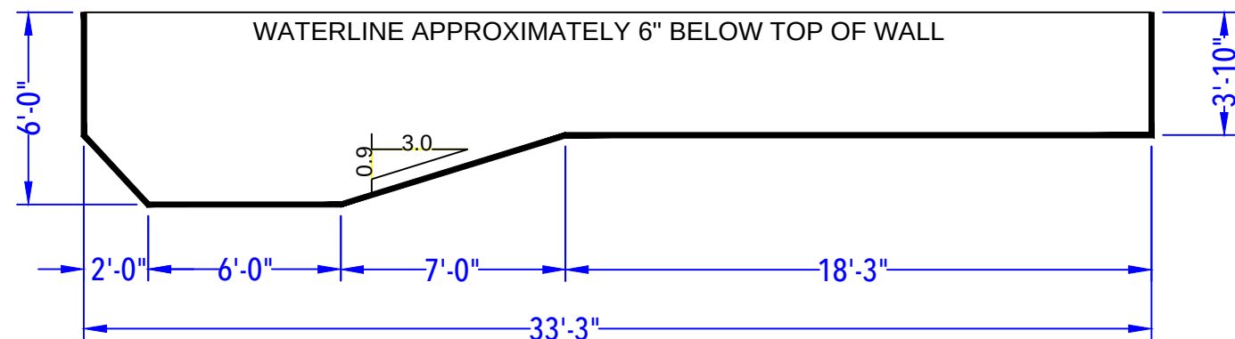
DEPTH DETAIL
