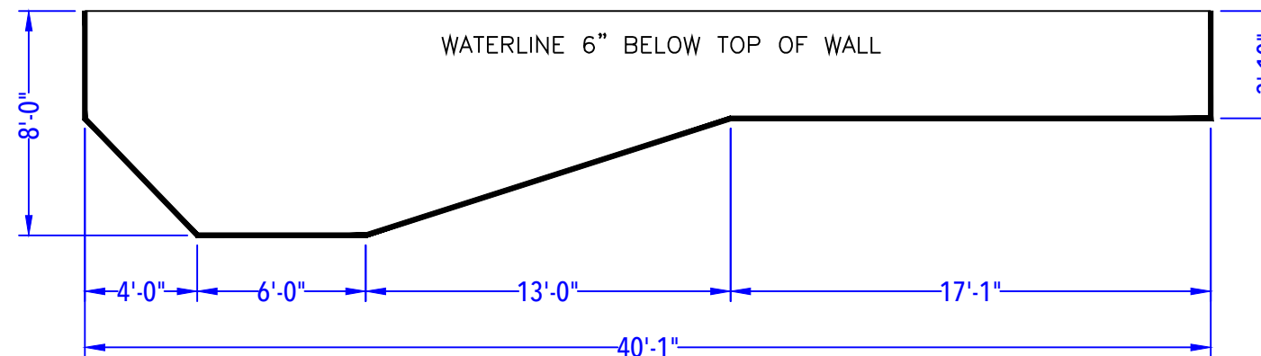
DEPTH DETAIL
