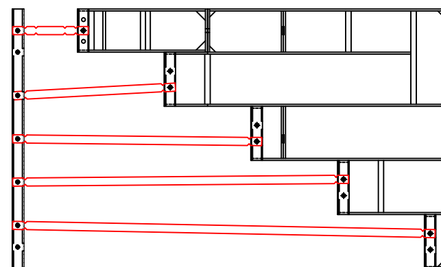
8'-4" Outside End Step - 24" Radius Corners
