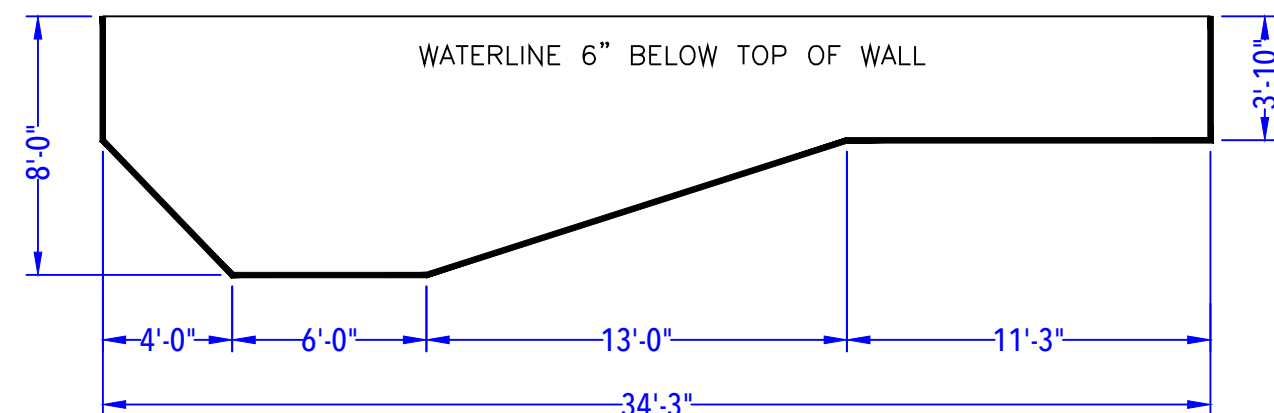
DEPTH DETAIL
