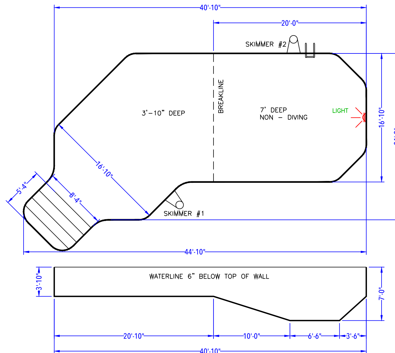
DEPTH DETAIL
