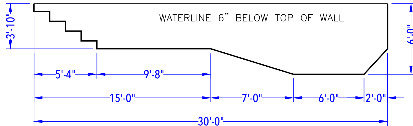
DEPTH DETAIL
