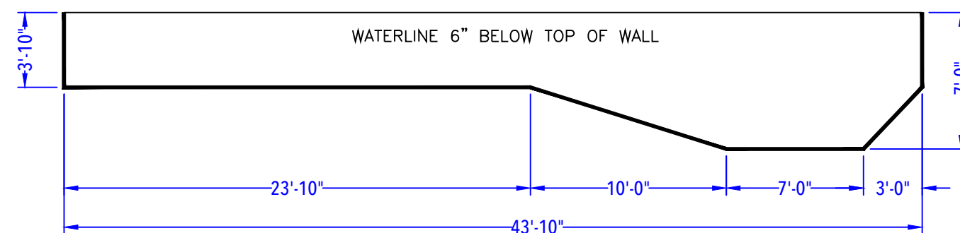
DEPTH DETAIL
