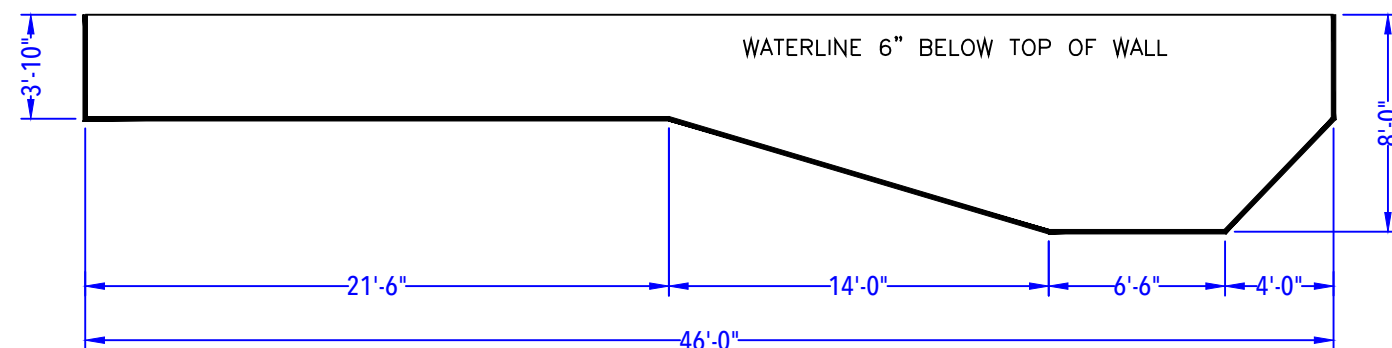
DEPTH DETAIL
