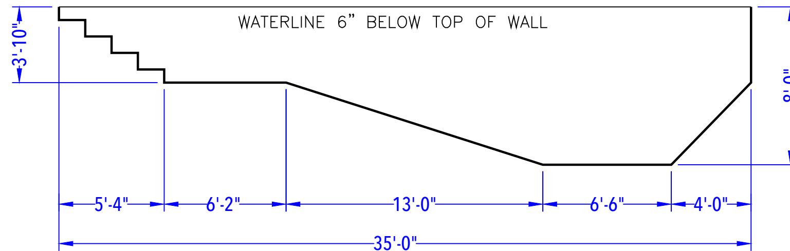
DEPTH DETAIL
