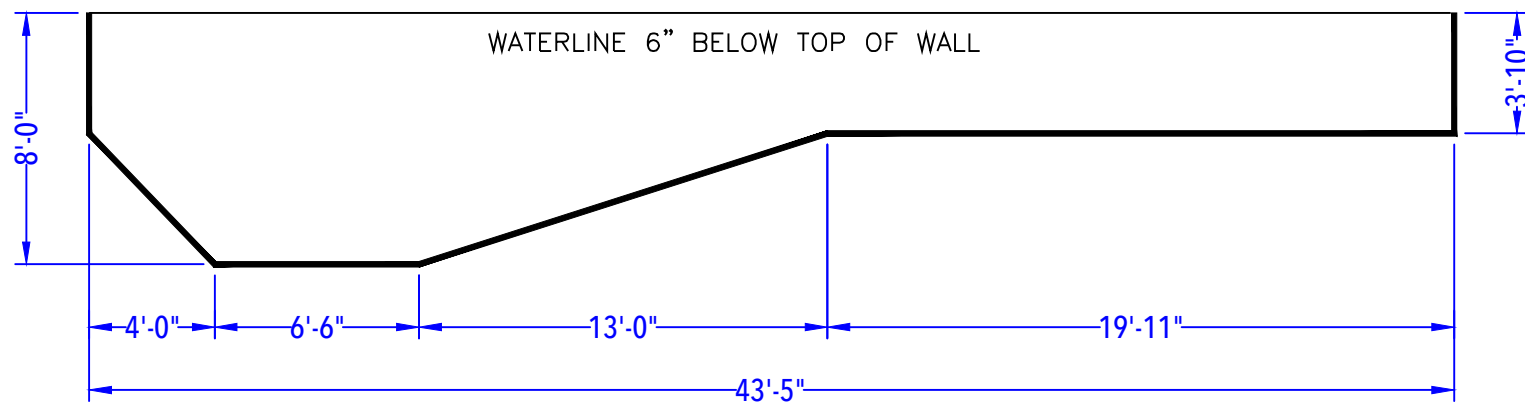
DEPTH DETAIL
