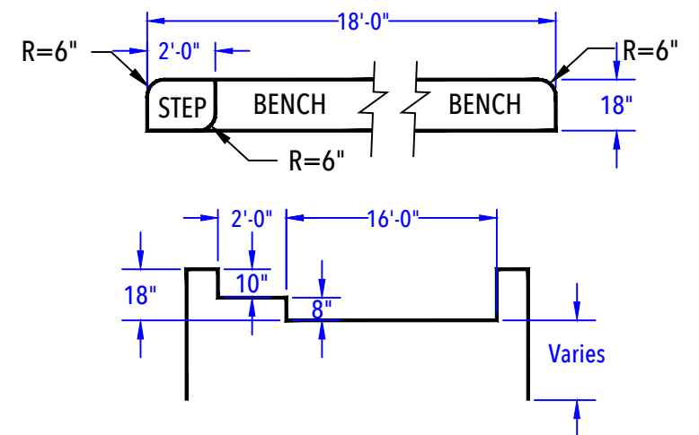
DEEP END BENCH & STEP OUT DETAIL (After Concrete & Liner) N.T.S.
