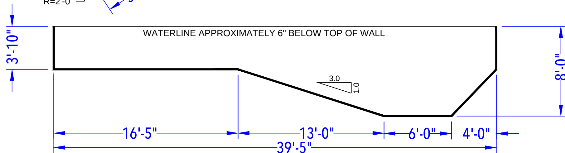
DEPTH DETAIL
