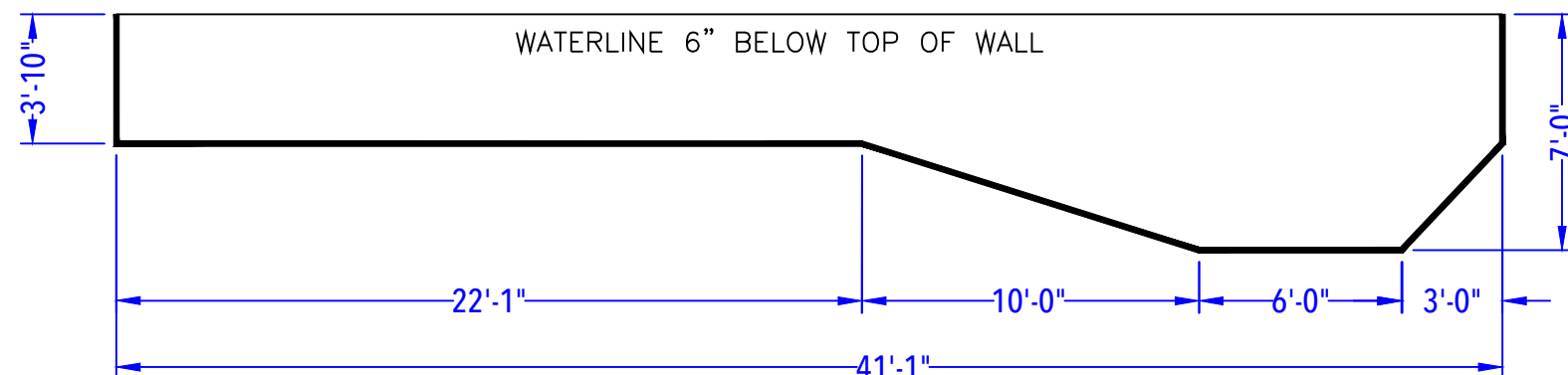
DEPTH DETAIL
