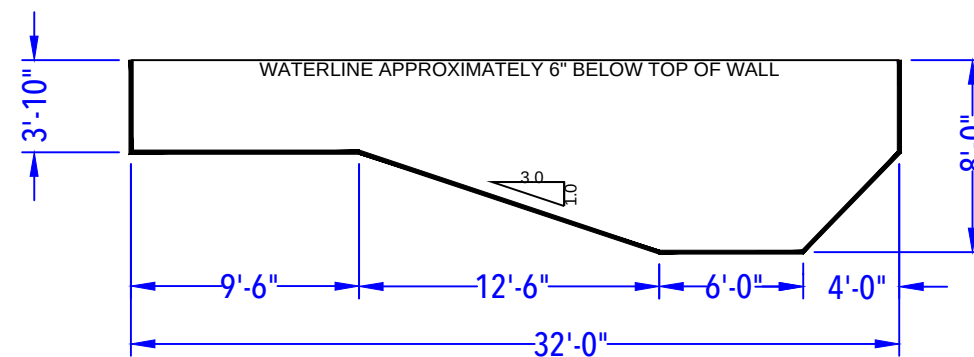
DEPTH DETAIL
