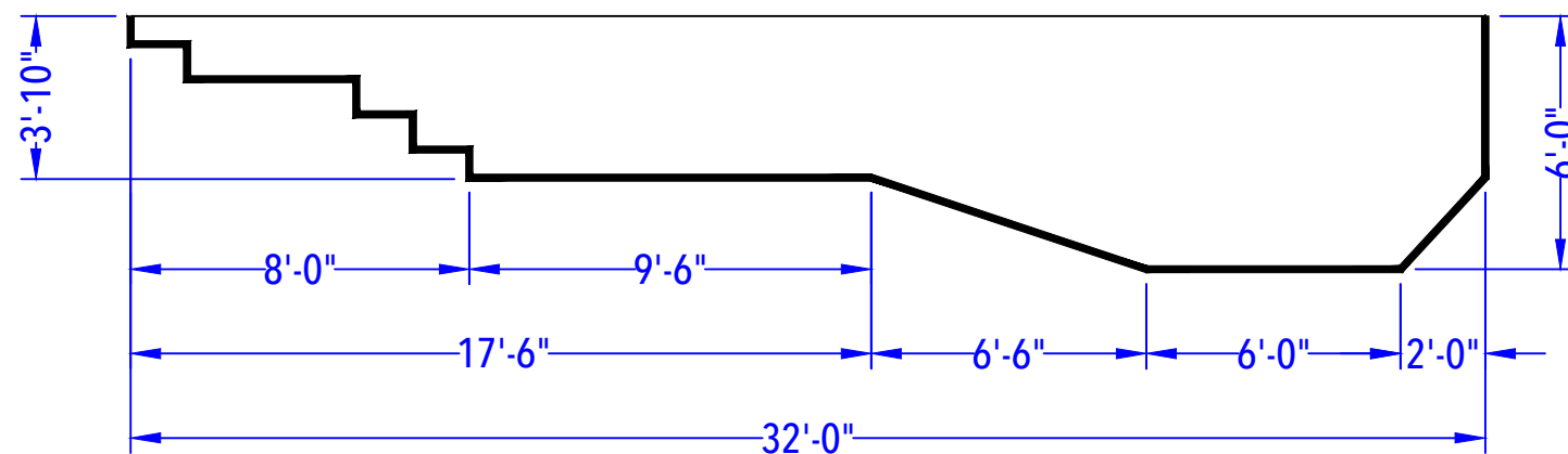
DEPTH DETAIL
