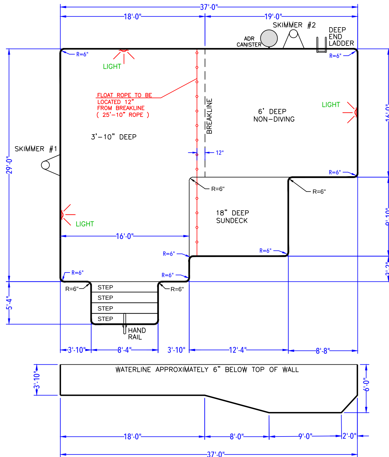
DEPTH DETAIL
