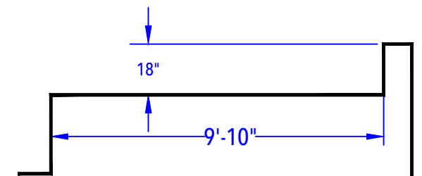
SIDE SUN DECK DETAIL (After Concrete & Liner) N.T.S.
