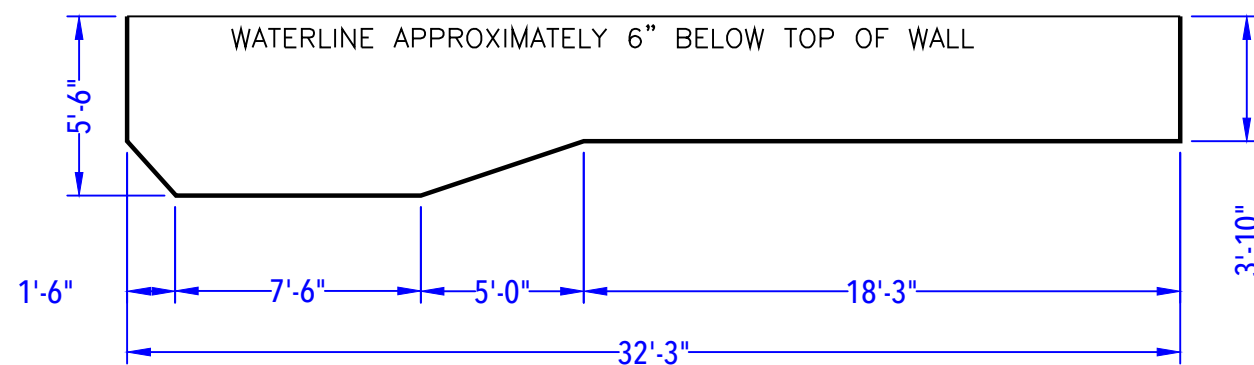
DEPTH DETAIL
