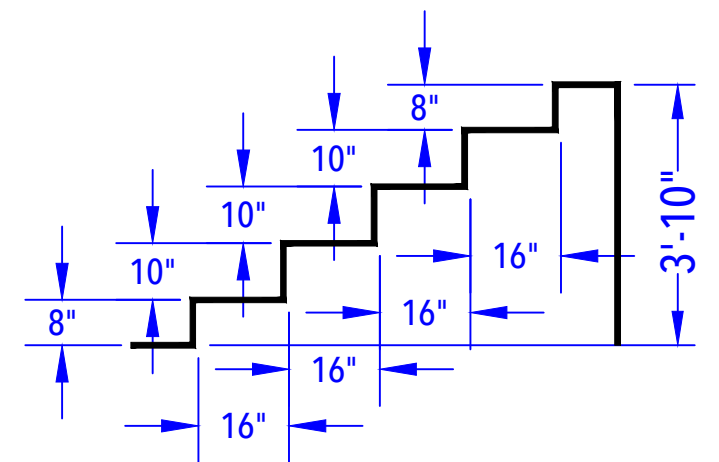
ENTRY STEP DETAIL (After Concrete & Liner) N.T.S.
