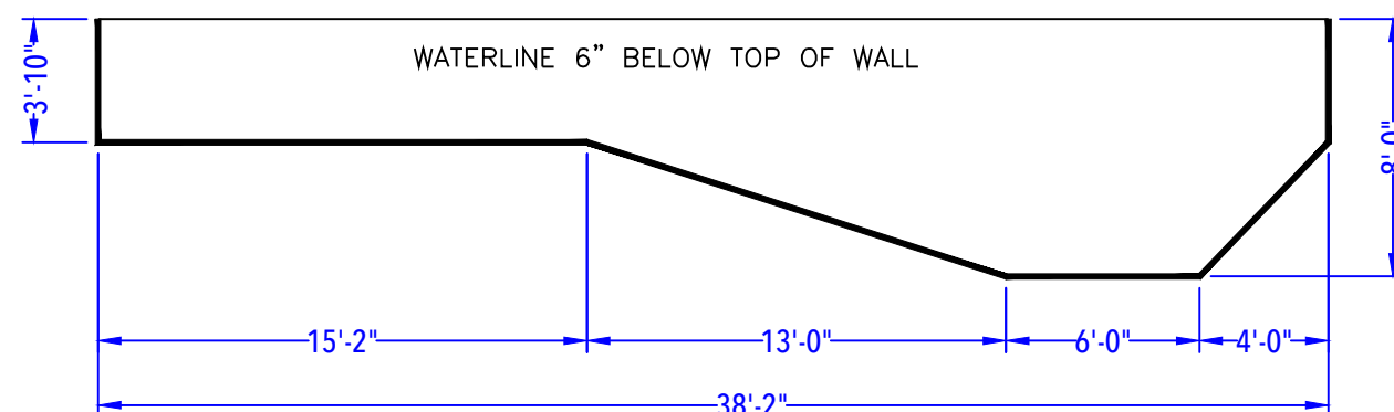
DEPTH DETAIL
