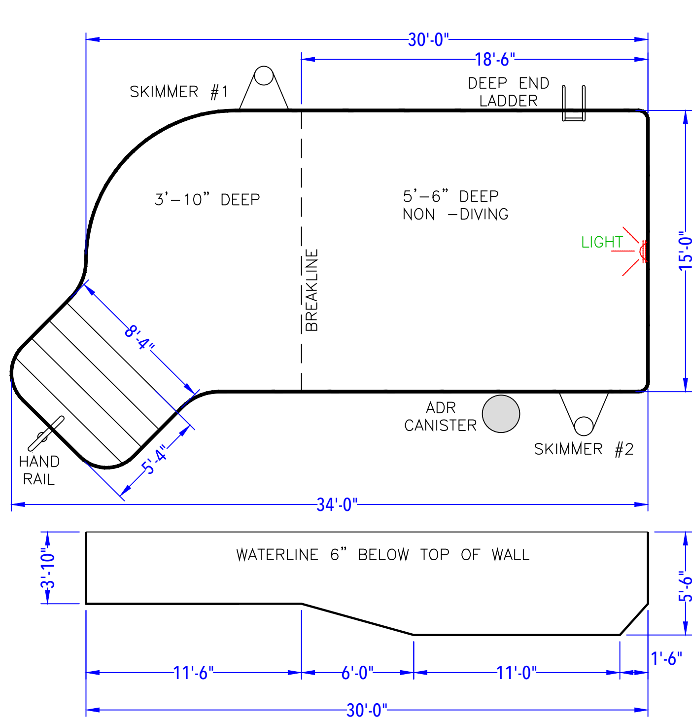
DEPTH DETAIL
