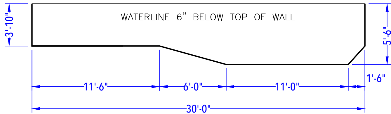
DEPTH DETAIL
