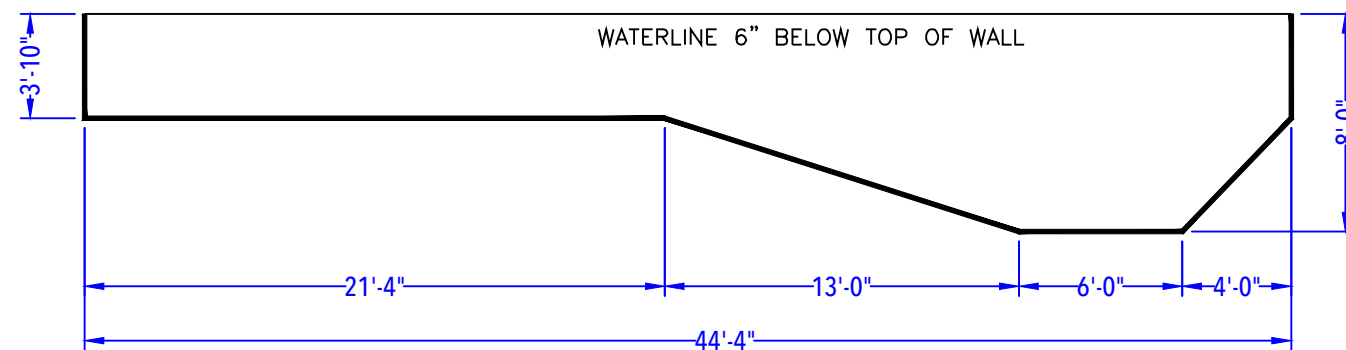
DEPTH DETAIL
