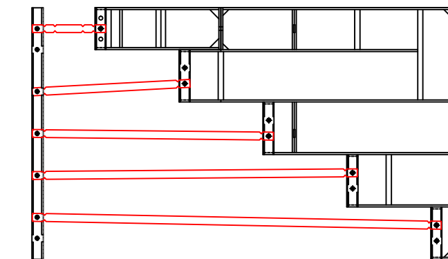
8'-4" x 5'-4" Outside End Step - 6" Radius Corners
