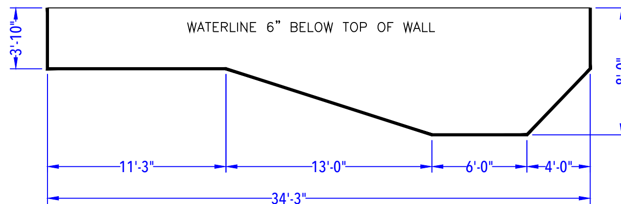
DEPTH DETAIL
