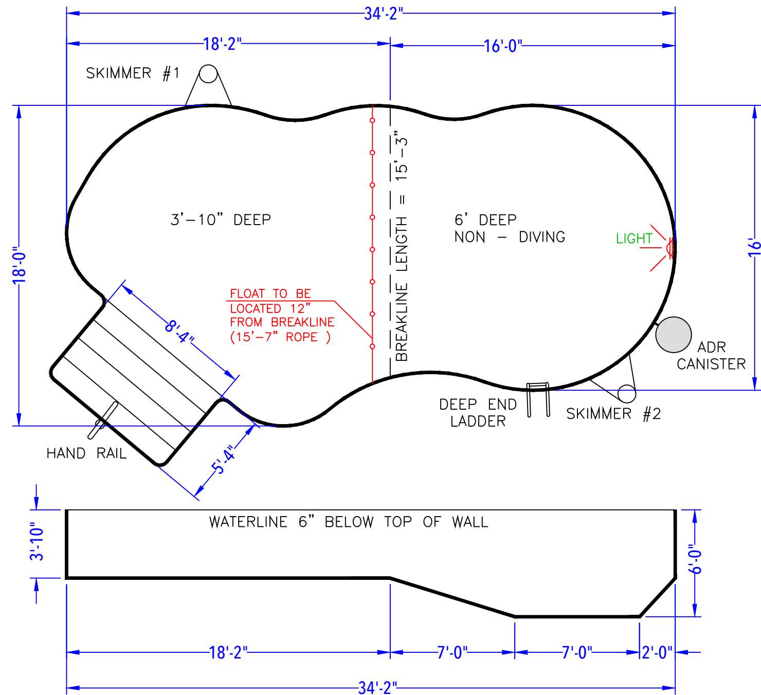
DEPTH DETAIL
