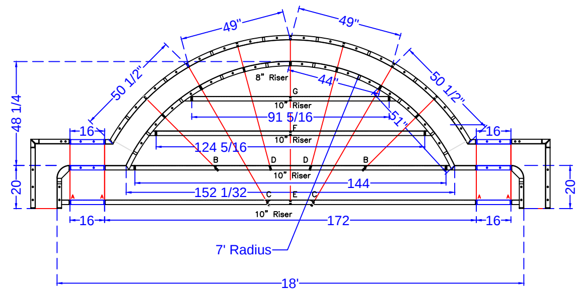
18' ROMAN END STEP ASSEMBLY SHOWN x 48 SCALE: 1' = 1/4"
