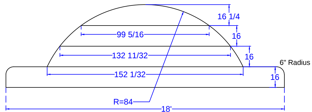
STEP DETAIL SCALE: 1' = 1/4"
