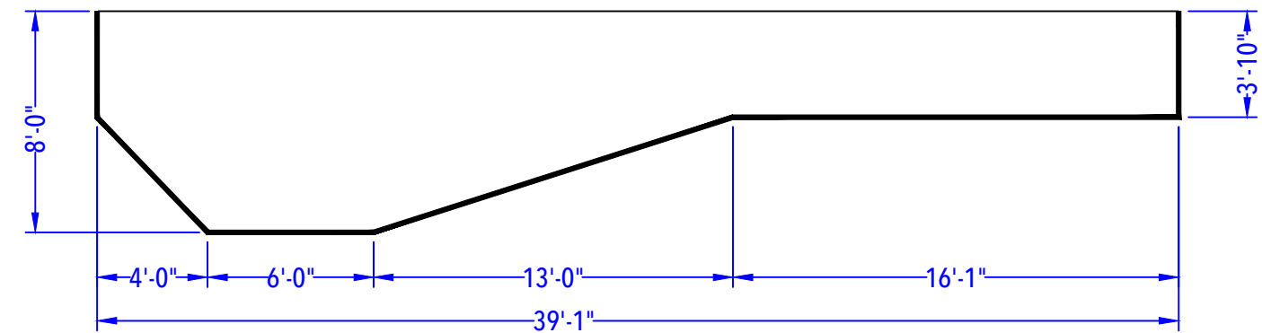
DEPTH DETAIL
