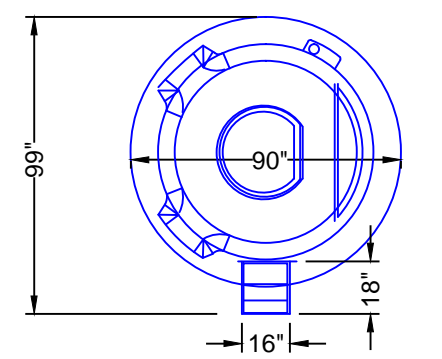
90" ROUND FIBERGLASS SPILLOVER SPA DETAIL (After Concrete & Liner) N.T.S.
