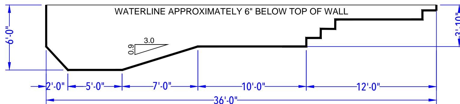
DEPTH DETAIL
