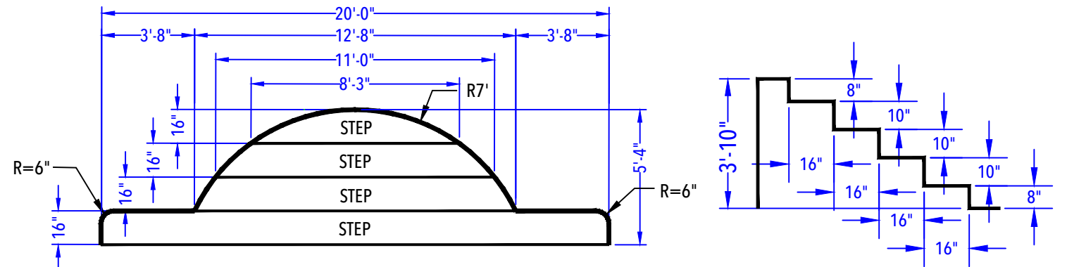
ENTRY STEP DETAIL (After Concrete & Liner) N.T.S.
