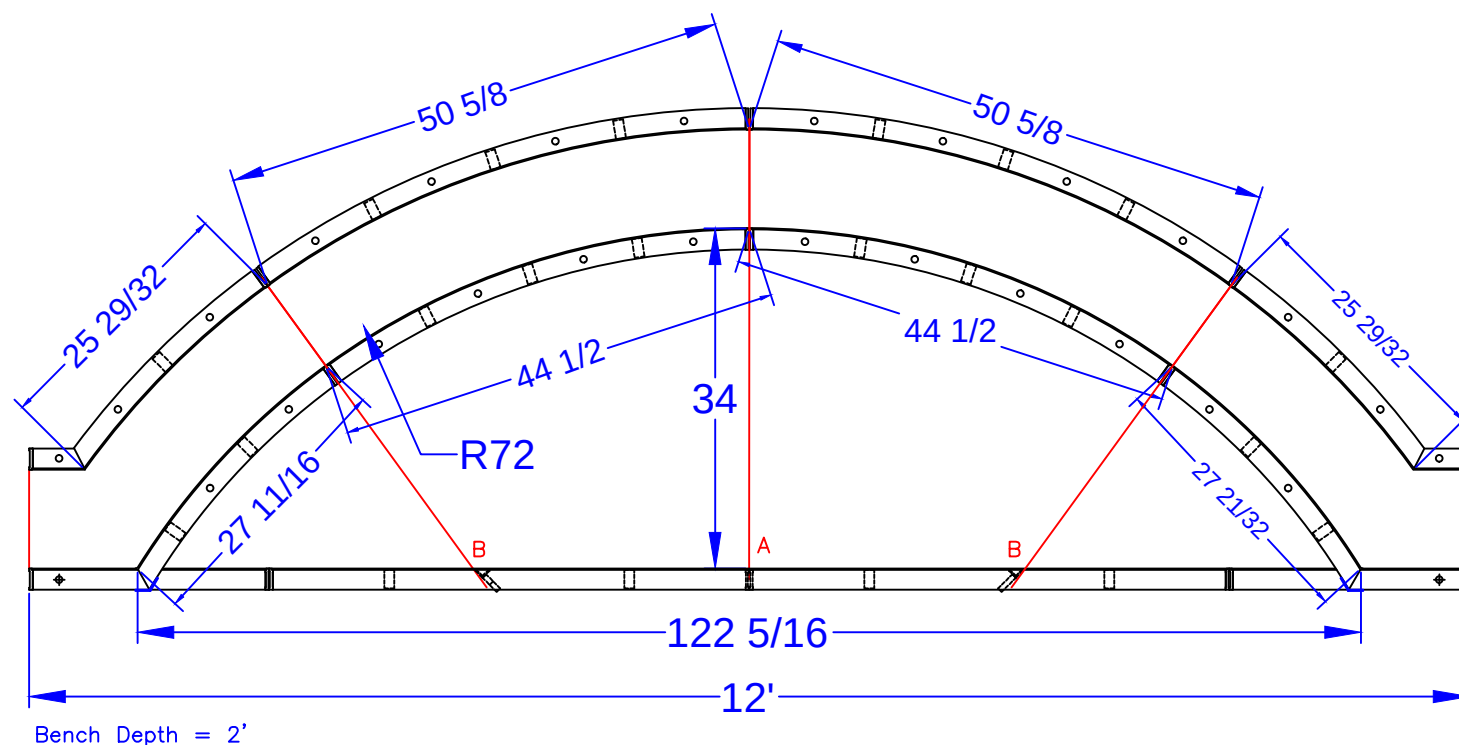
44" Full Pool Tie 1/4" BB DRN
