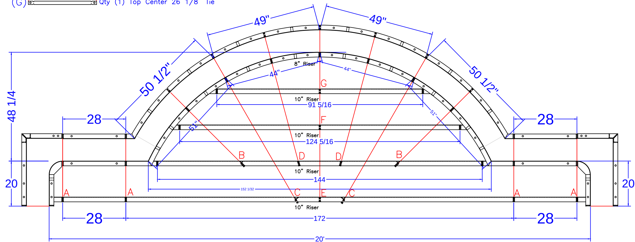
20' WIDE ROMAN END STEP DETAIL
