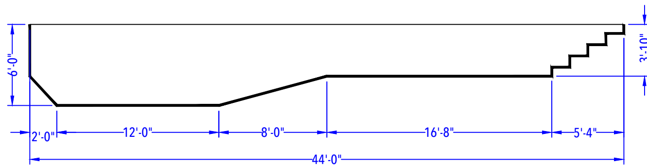
DEPTH DETAIL
