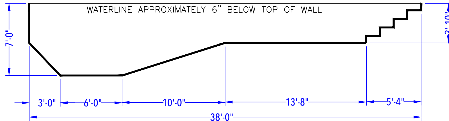
DEPTH DETAIL
