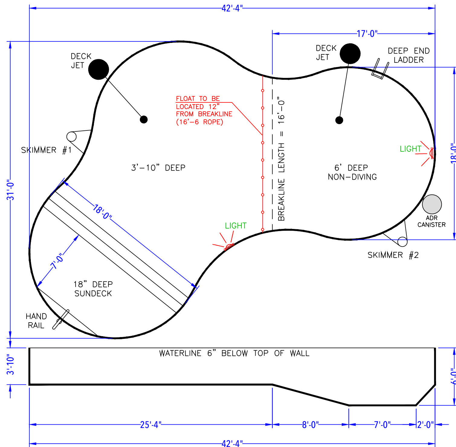
DEPTH DETAIL
