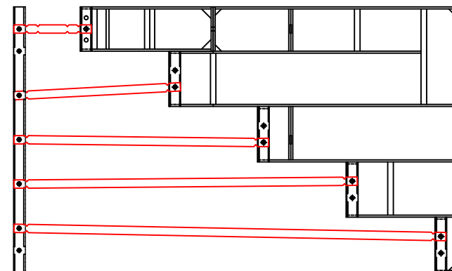
6'-4" x 5'-4" Outside End Step - 6" Radius Corners
